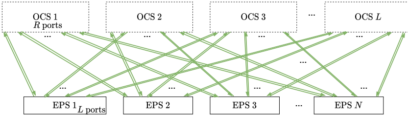
Fig. 2. \mathcal{G}_{\text{uniform}} topology.
